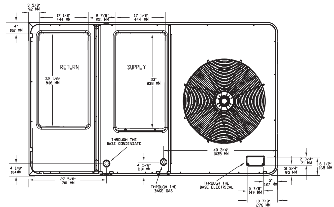
6 1/4 through 10 Ton Downflow Unit Supply & Return Air Openings
