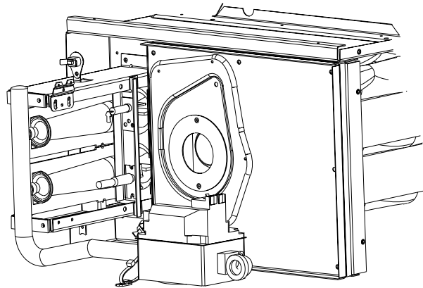
Figure 8 Typical Unit Gas Train Configuration
