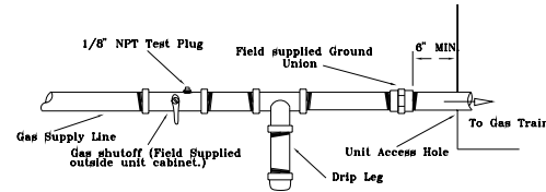
Figure 8 Typical Unit Gas Train Configuration
